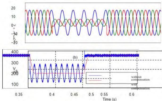
FIGURE 3. PV SYSTEM RESPONSE TO VOLTAGE DIP IN GRID
